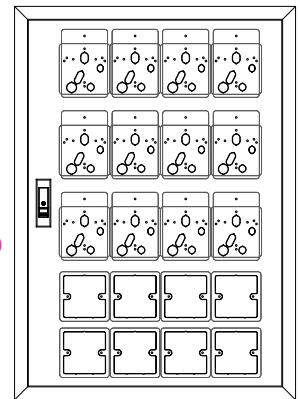
YRSB 50x70x6 - 12R8S
