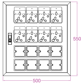
YRSB 50x55x6 - 8R8S
