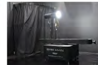
High Accuracy Goniophotometer
