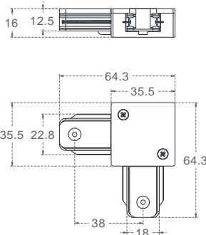
L Joint
