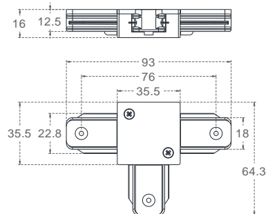
T Joint
