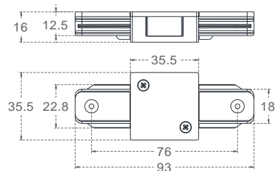
I Joint
